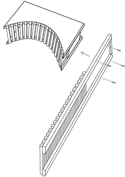
1 ATTACH RIGHT SIDE ASSEMBLY
