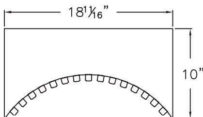
ARCH BODY
