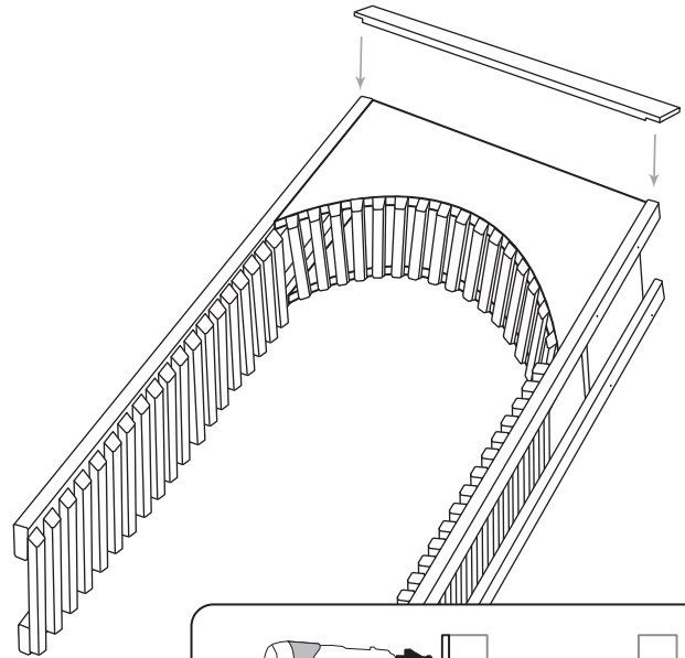
4 ATTACH TOP TRIM PIECE
