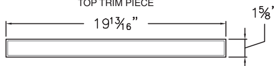
TOP TRIM PIECE
