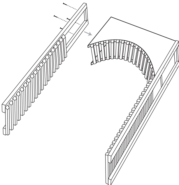
2 ATTACH LEFT SIDE ASSEMBLY
