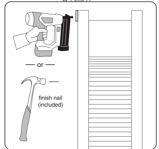
5 SECURE WITH FINISH NAILS
